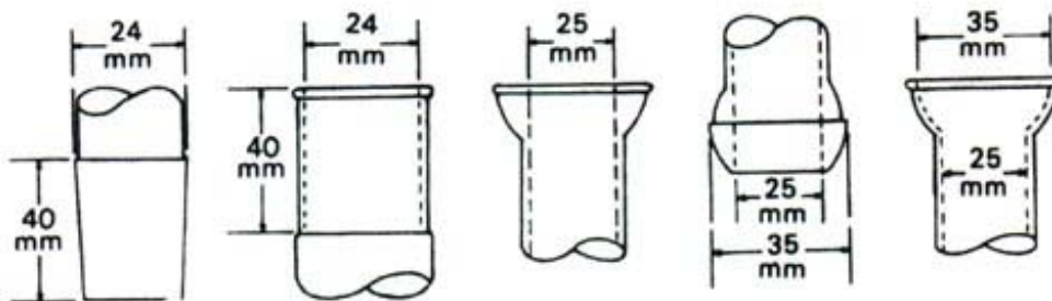
§ 24/40 Inner Joint
